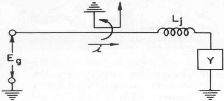
Figure 5c. Revised circuit of Figure 5b, with junction inductance shifted to the load side of the coupling loop.
