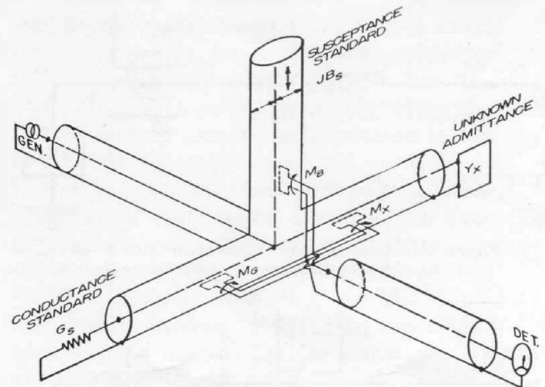
Figure 4. Schematic diagram of the Admittance Meter, showing the arrangement of coupling loop.
