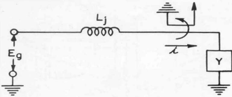
Figure 5b. Approximate equivalent circuit of each branch with junction capacitance neglected.
