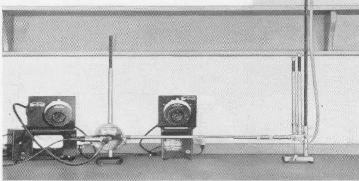
Figure 2. View of the Admittance Meter and balun as assembled for the measurement of a balanced transmission line.
