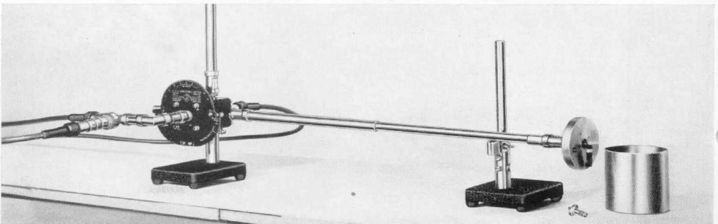
Figure 3. View of the Admittance Meter as set up for measurement of a resistor, showing the line stretcher and component mount.
