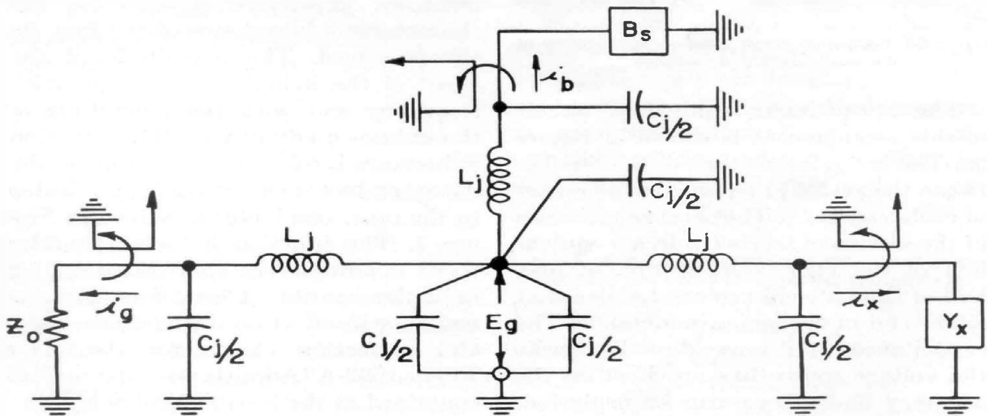
Figure 5a. Equivalent circuit of the junction.
