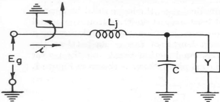
Figure 5d. Equivalent circuit showing the location of the compensating capacitance.
