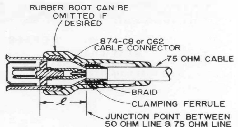
Figure 1. Sketch of Type 874-C63 Cable Connector with a 75-ohm cable attached.
