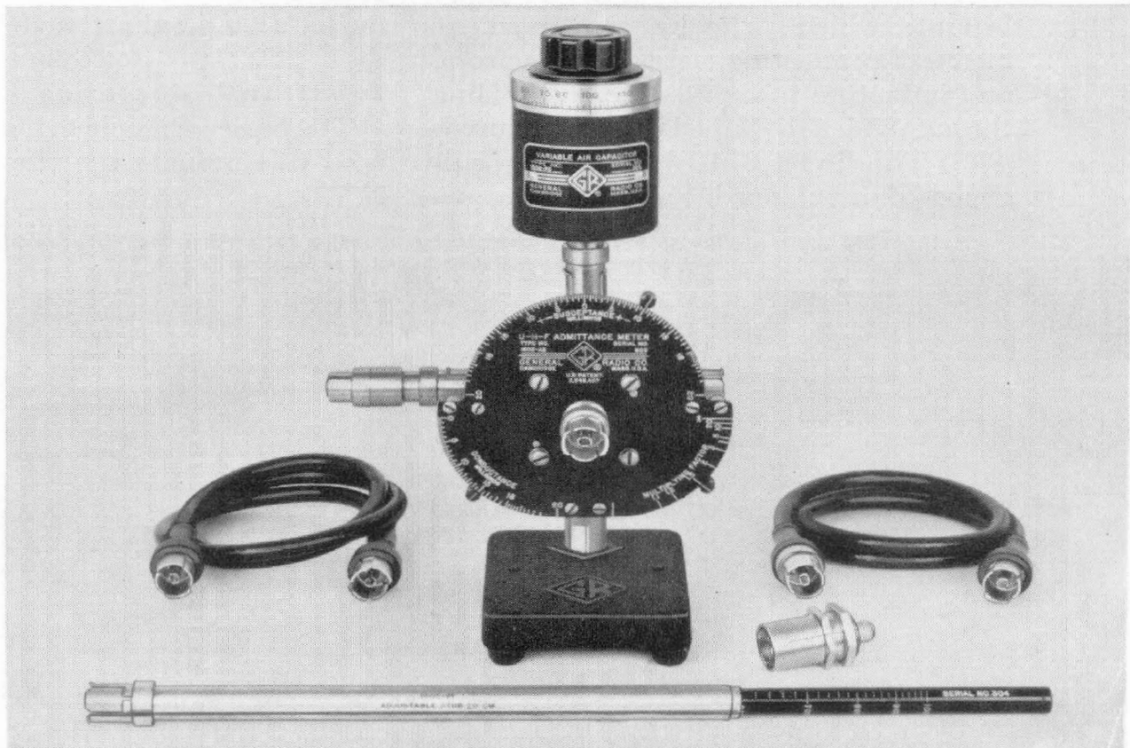
Figure 1. Close-up of the Type 1602-B U-H-F Admittance Meter.
