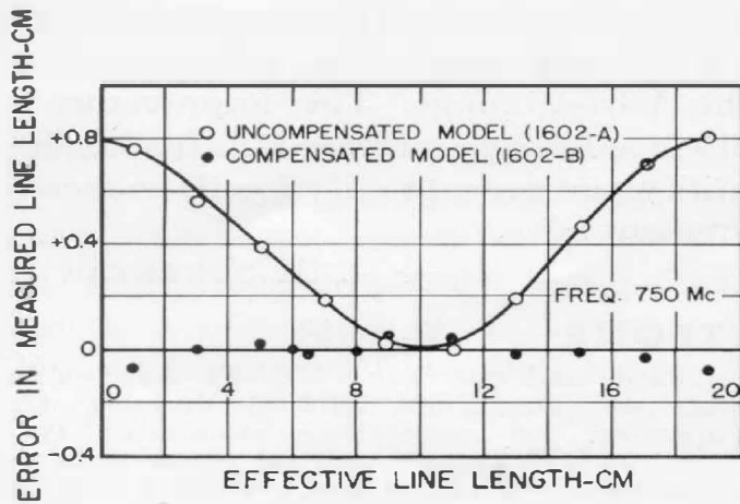
Figure 6. Curves showing the error in measured length of a short-circuited line as a function of its electrical length when the junction inductance is ignored, as measured by both the older, uncompensated Type 1602-A Admittance Meter and the new Type 1602-B compensated model.
