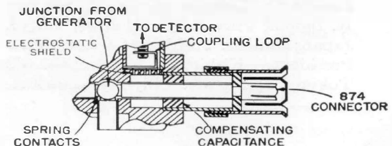
Figure 7. Sketch of modified junction showing the location of one of the compensating capacitances.
